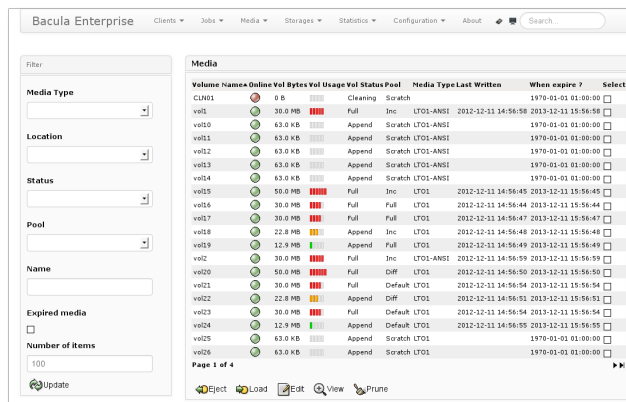
Figure 3: Volume Information
