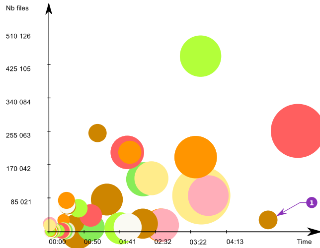
Figure 6: Statistics Module
