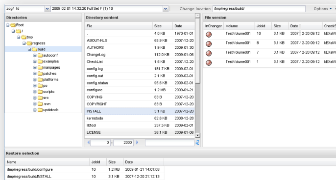
BWeb Management Suite restore interface
